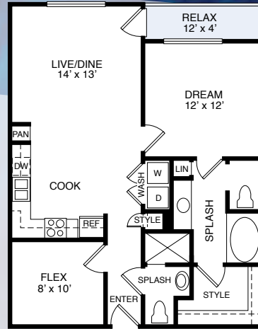
PLAN A1 1 Bedroom+Flex, 2 Bath 864 sq. ft.
